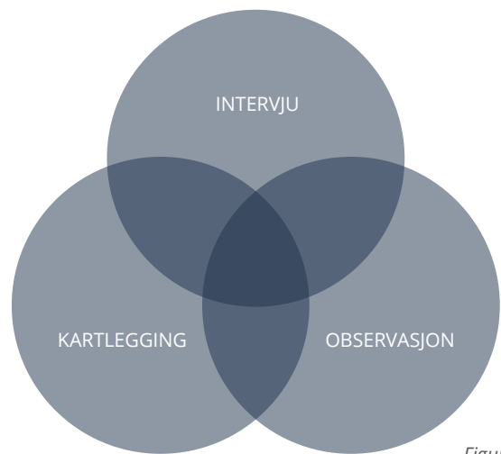
Figur 4.3: Metodetriangulering.
